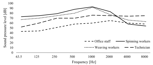
Fig. 2. Frequency analysis of emitted noise in octave band.
