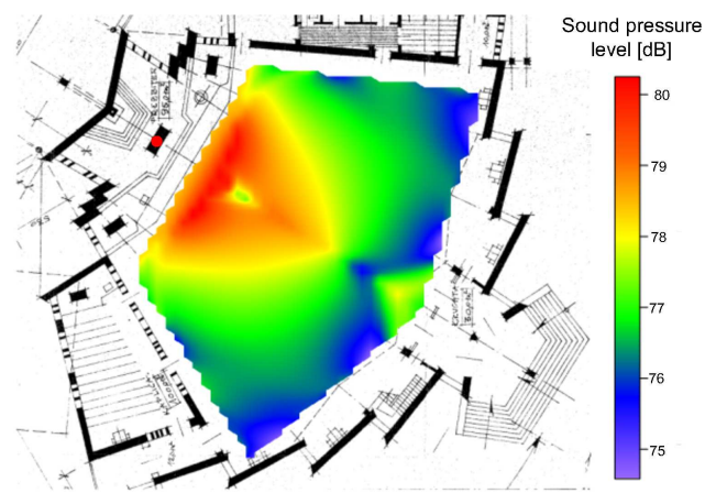
Fig. 10. Distribution of sound pressure level SPL, the church of the VM.
