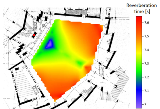
Fig. 11. Distribution of reverberation time T_{30} , the church of the VM.
