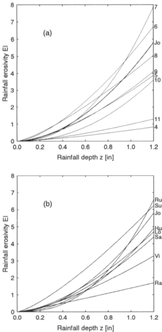
Fig. 3. Least-square fitted power-laws (see Eq.5) for computing daily rainfall erosivity EI [(100 ft-tonsf/acre)(in/h)] as a function of daily rainfall amount [in]. (a) for the months April-November (4-11) and the whole observation period (Jo; thick line) in Jokioinen, (b) for the whole observation period at the 8 stations.
