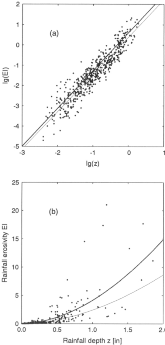
Fig. 2. Rainfall erosivity EI [(100 ft-tonsf/acre)(in/h)] as a function of daily rainfall amount [in] in Jokioinen (a) in double-logarithmic scale, (b) in normal scale. The thin line shows the least-square fit obtained by linear regression of the log-transformed data, and the thick line shows the least-square fit obtained by non-linear regression on the original data.
