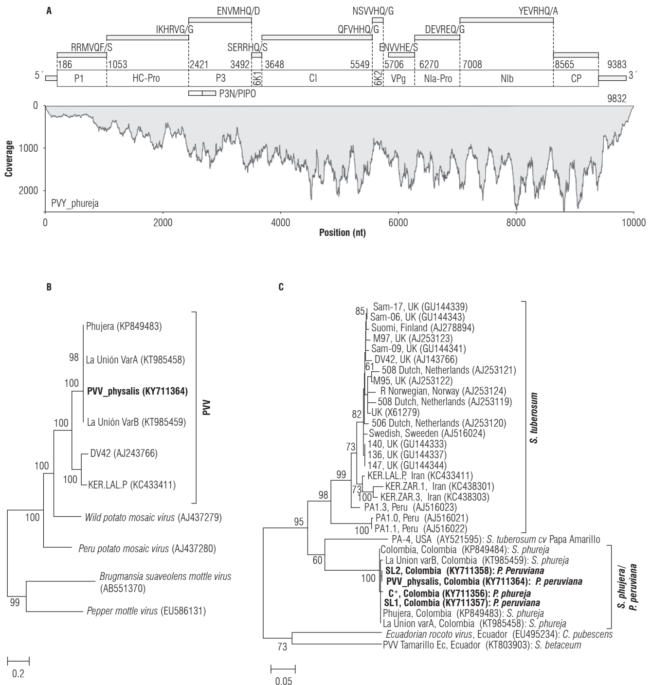
FIGURE 3. Genome annotation of the PVV_phureja genome and phylogenetic relationship to other PVV isolates. A ) Sequence coverage of PVV_phureja assembly and location of some important molecular features. The relative position of each mature protein with their corresponding protease cleavage sites is shown. Phylogenetic analysis of PVV isolates using complete (B) and partial CP (C) sequences confirms the close relationship between PVV_physalis and PVV isolates infecting S. phureja . Trees are drawn to scale with branch lengths in units of number of base substitutions per site as indicated in the bar at the bottom. Bootstrap values are shown above the branches.
