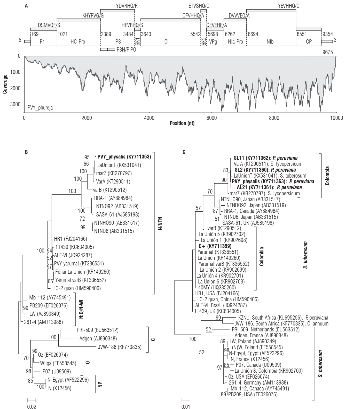
FIGURE 2. Genome annotation of the PVY_phureja genome and the phylogenetic relationship to other PVY isolates. A ) Sequence coverage of PVY_phureja assembly and location of some important molecular features. The relative position of each mature protein with their corresponding protease cleavage sites is shown. Phylogenetic analysis of PVY isolates using complete (B) and partial CP (C) sequences confirms the close relationship between PVY_physalis and non-recombinant PVY isolates infecting S. lycopersicum and S. tuberosum in eastern Antioquia. Trees are drawn to scale with branch lengths in units of number of base substitutions per site as indicated in the bar at the bottom. Bootstrap values are shown above the branches.
