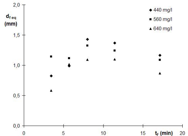
FIGURE 2. Experimental data — Maximum flock size vs. flocculation time — d_{f,eq} = f(t_F) .
