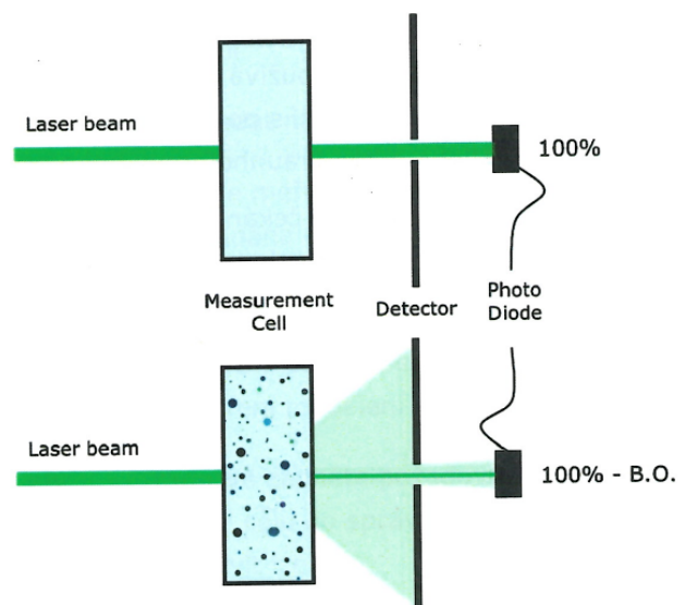
FIGURE 2. Concept of laser beam shielding
