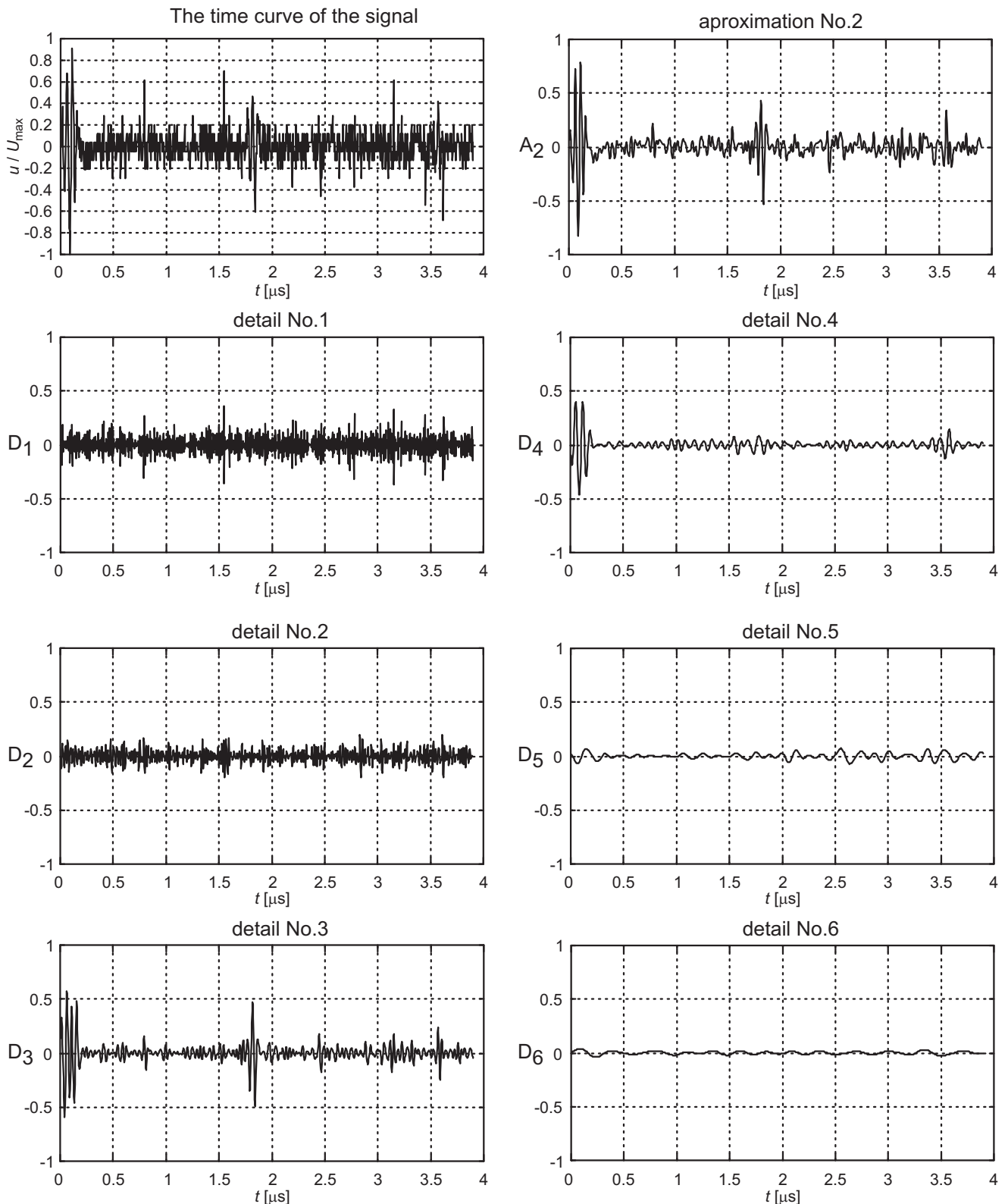
Fig. 3: Decomposition of the simulated signal for \ell=6 (drawings of all details of the wavelet analysis and one selected approximation)
