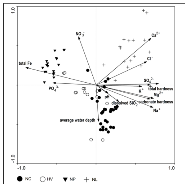
Fig. 1 CCA ordination diagram of 1st and 2nd axes obtained for water properties and relevés of four plant communities, dominated by: NC – Nymphaea candida ; HV – Hydrilla verticillata ; NP – Nuphar pumila ; NL – Nuphar lutea . Eigenvalues: \lambda_1 = 0.787 ; \lambda_2 = 0.595 ; \lambda_3 = 0.216 ; \lambda_4 = 0.108 . Monte Carlo permutation test of significance of all canonical axes: p = 0.002 .
