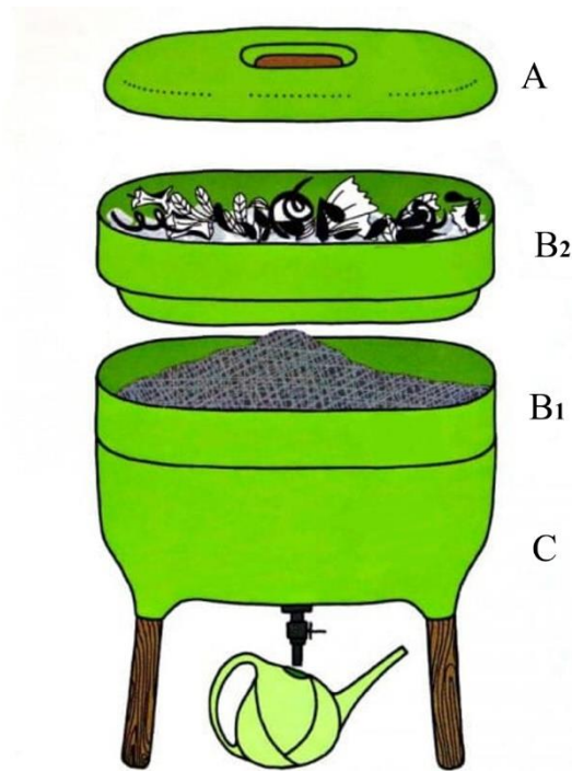
Fig. 5. Scheme of an exemplary gazebo composter: A – cover, B1, B2 – chambers for bio-waste and earthworms, C – lower chamber for liquid fertiliser (Source: Public domain, changed)
