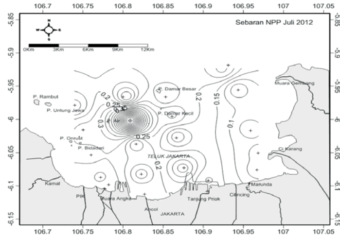
Figure 8. NPP distributions in Jakarta Bay based on field measurement on July 2012
