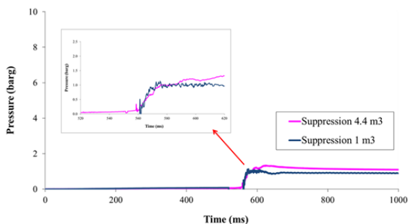
Figure 3: 4.4 m 3 vessel (FSA) used for the suppression tests and comparison of the explosion pressure curves from 1-m 3 and 4.4-m 3 suppression tests with 500 g/m 3 of aluminum dust (Taveau et al., 2015)
