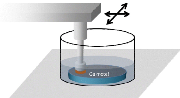
Figure 1: Scheme of the experimental apparatus adopted in the present study. The orange disc is the abrasive fabric pad
