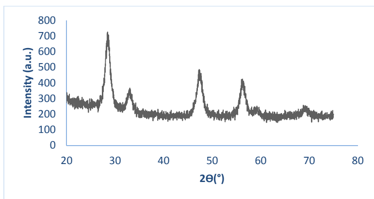
Figure 3. XRD analysis of experiment 4 calcined
