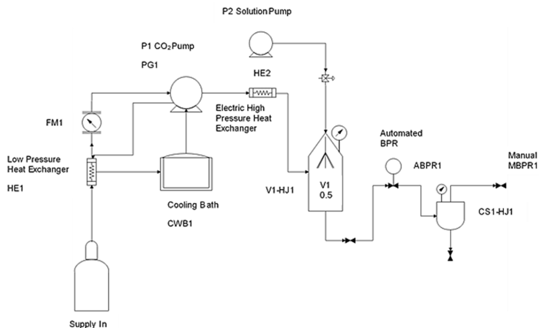
Figure 1. Schematic diagram SAS200 lab-scale plant
