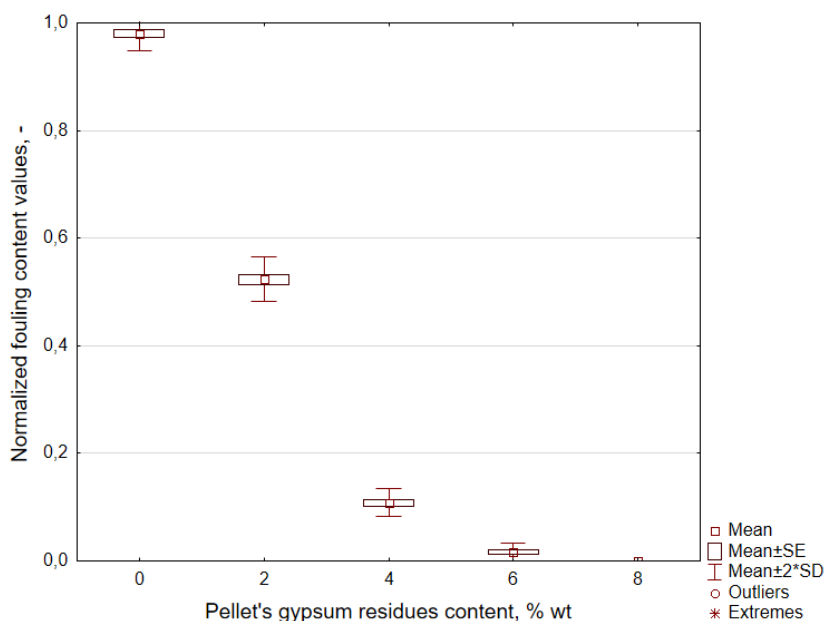
Figure 5: Normalized fouling content produced by the pallet's burning as a function of the percentage of hydrated gypsum
