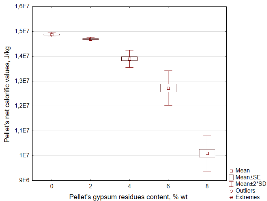
Figure 4: Net calorific value of Pellet's macrophytes as a function of the content of hydrated gypsum residues
