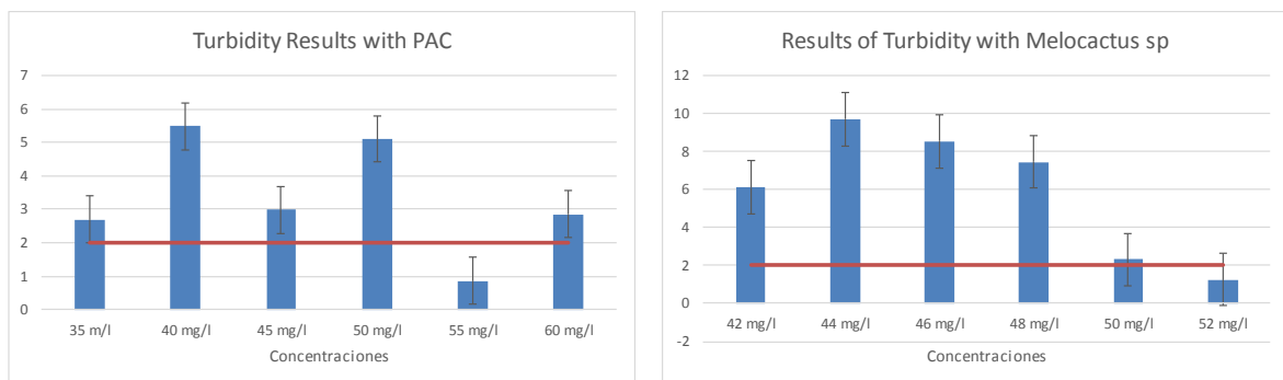
Figure 3: Results of the turbidity analysis of the waters with PAC and with extract of Melocactus sp
