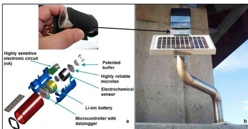
Figure 3: (a) Photography of a Caisens and schematic representation of its main components, (b) Photography of the autonomous wireless measurement point.
