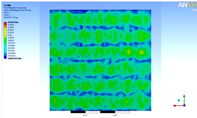
Figure.3: Total magnetic flux density on plastic surface
