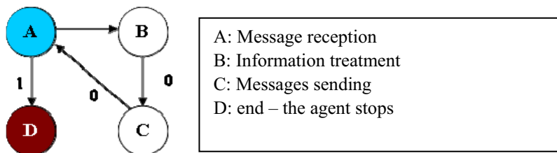
Figure 2: Behavior of the Information and Evaluation-Anticipation Agents
