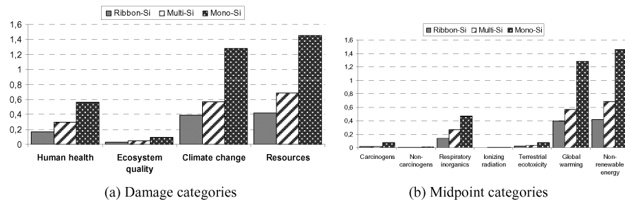
Figure 2: Normalized results of LCA for the three technology modules
