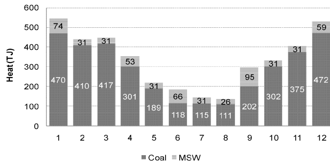
Figure 4: Heat production throughout the year
