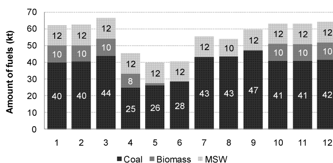
Figure 3.: Coal, biomass and MSW utilization throughout the year
