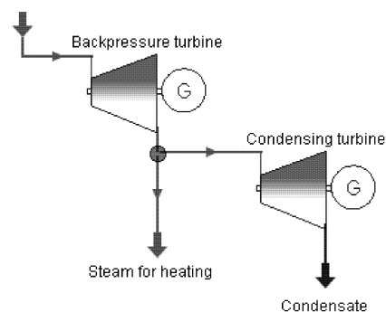
Figure 1: Schema of the turbine house in WTE plant
