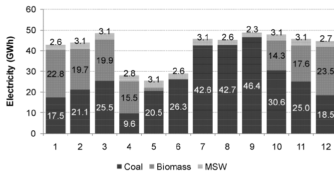
Figure 5: Electricity production throughout the year
