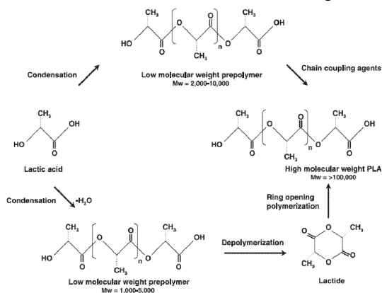
Figure 1: PLA synthesis methods (Gupta et al, 2007)
