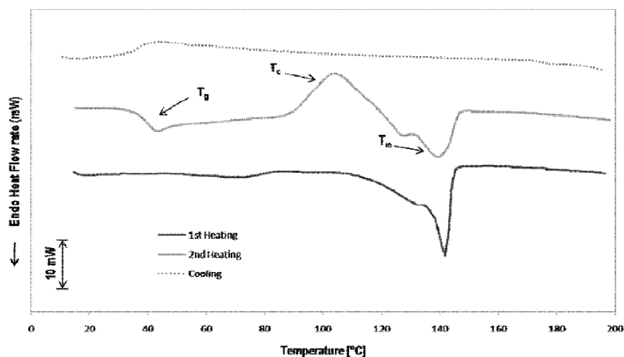
Figure 3: DSC thermogram
