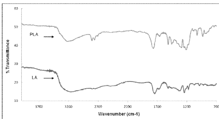
Figure 4: FTIR of PLA and lactic acid
