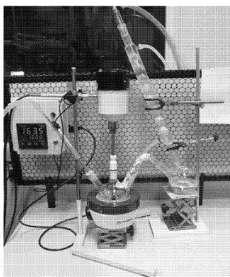
Figure 2: Polymerization experimental system
