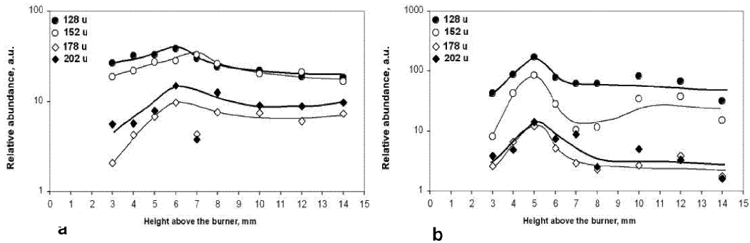
Figure 3. Axial profiles of the most abundant PAH (128u, 152u,178u, 202u) at C/O=0.6 (a) and at C/O=0.65 (b).
