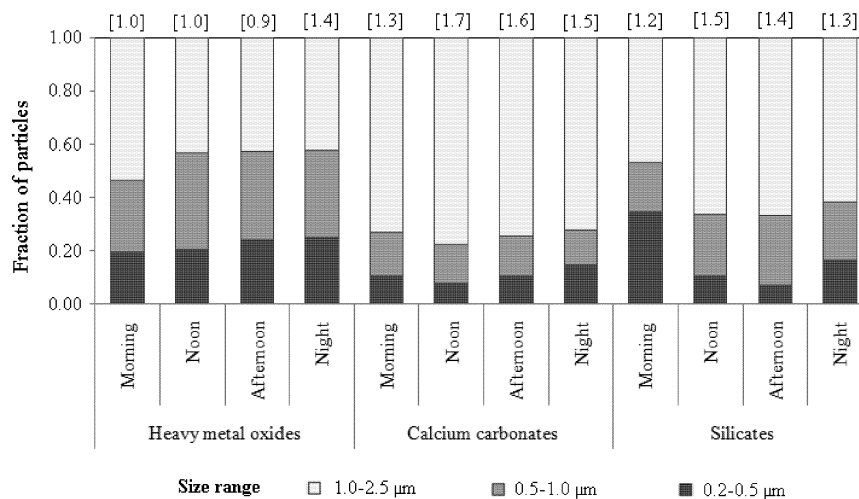
Figure 1. Fraction of particles in the 0.2-0.5 \mu\text{m} (dark grey), 0.5-1.0 \mu\text{m} (medium grey), 1.0-2.5 \mu\text{m} (light grey) in each cluster and period. Particle mean size placed in the top of the bar in brackets.
