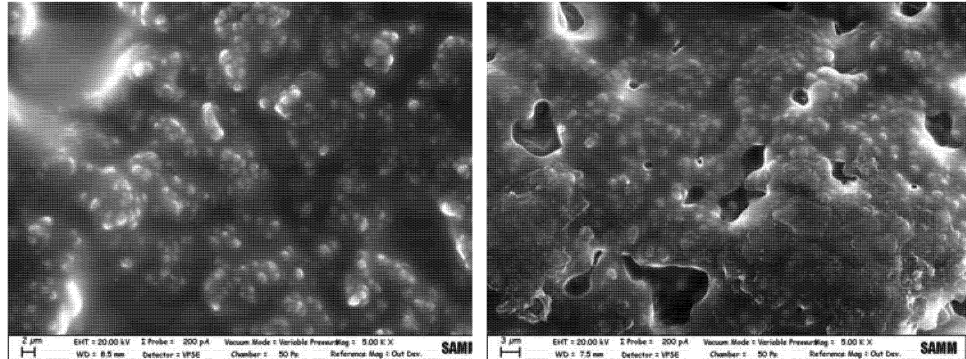
Fig. 3. Sol gel films over Al and Mg-oxide from anodisation, obtained at ambient temperature. The nanosized structure strongly decreases at high temperature [Amoriello,2009].
