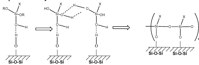
Fig. 1 . Organosilanes condensation over metal oxide. first step: adsorption, second step: hydrolysis with silanols formation, third step: condensation with covalent bonds formation and polymer. ( x = organic fragment) [Lamure].
