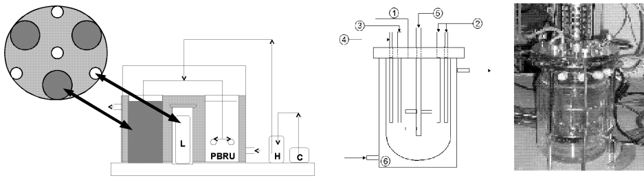
Figure 1. Equipment used in the experimentation. Left (a): Bubble-column photobioreactor; right (b): general-purpose, mechanically agitated fermenter .
