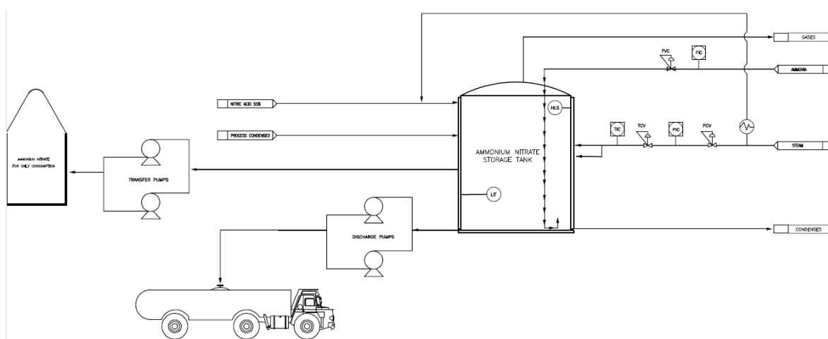
Figure 1. Production of Ammonium nitrate from gaseous Ammonia and Nitric acid.
