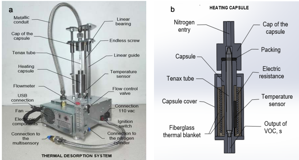
Figure 4: a) Thermal Desorption System. b) View of the transversal section of the de la capsule.
