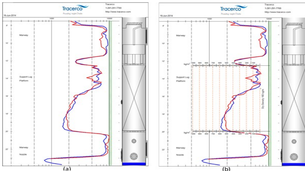
Figure 3. (a) Initial gamma scan results from small diameter column. (b) Gamma scan results, enhanced with liquid retention scale, showing missing packing at top of bed.
