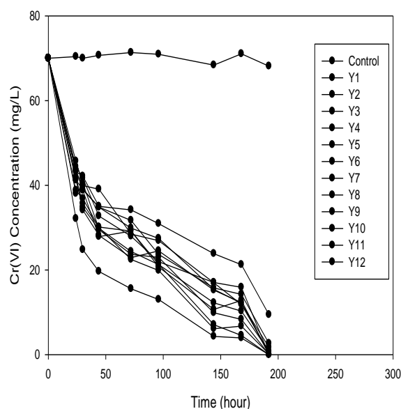
Figure 2: Cr(VI) removal efficiency of individual isolates
