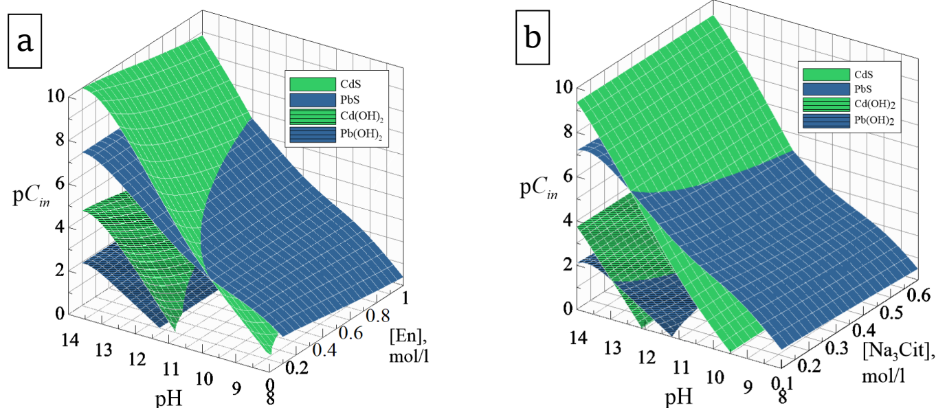
Fig. 1 Boundary conditions of the PbS, CdS, \text{Pb}(\text{OH})_2 and \text{Cd}(\text{OH})_2 sparingly soluble phases formation depending on the pH of the medium and the concentration of ethylenediamine (En) (a) and sodium citrate \text{Na}_3\text{Cit} (b). Calculations were performed at [\text{Na}_3\text{Cit}] = 0.3 \text{ mol/l} (a) and [\text{En}] = 0.6 \text{ mol/l} (b), T = 298 \text{ K}
