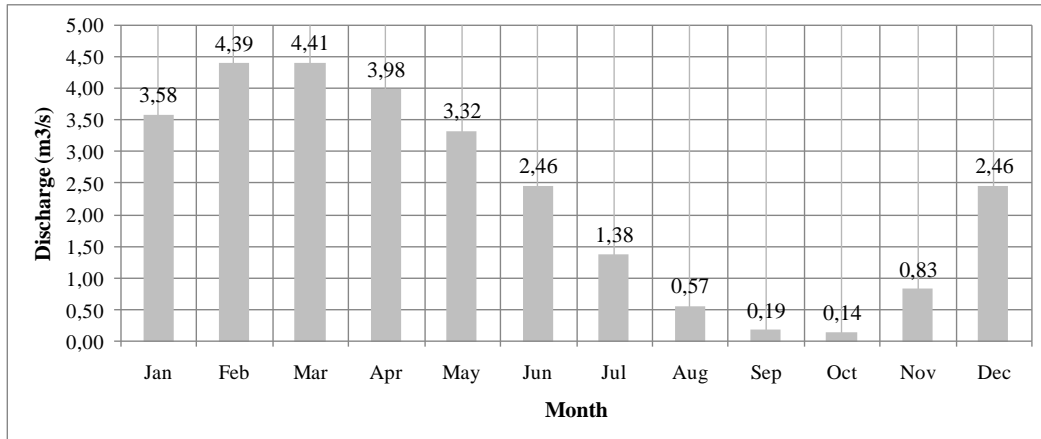
Figure 2. Dependable flow with 80% reliability of Pengubuan River
