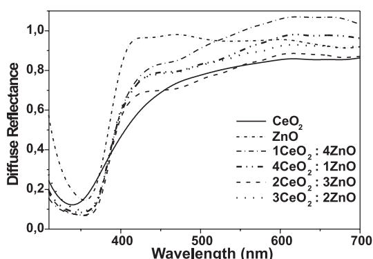
Figure 4. Reflectance spectra of CeO 2 , ZnO and the CeO 2 -ZnO nanopowder systems.
