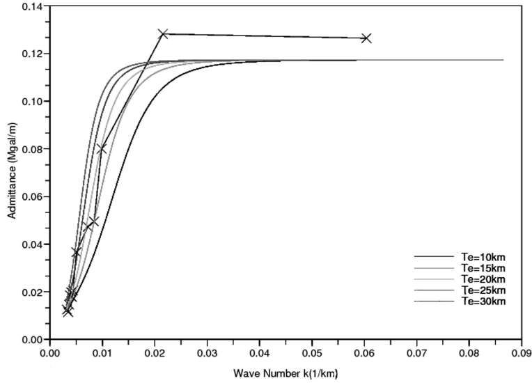
Figure 4: Theoretical admittance curves for T_e = 10, 15, 20, 25 and 30 km, and observed admittance curve. All the curves were calculated from topographical heights and free air gravity anomalies.
