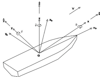
Fig.1. Motions and coordinate system
