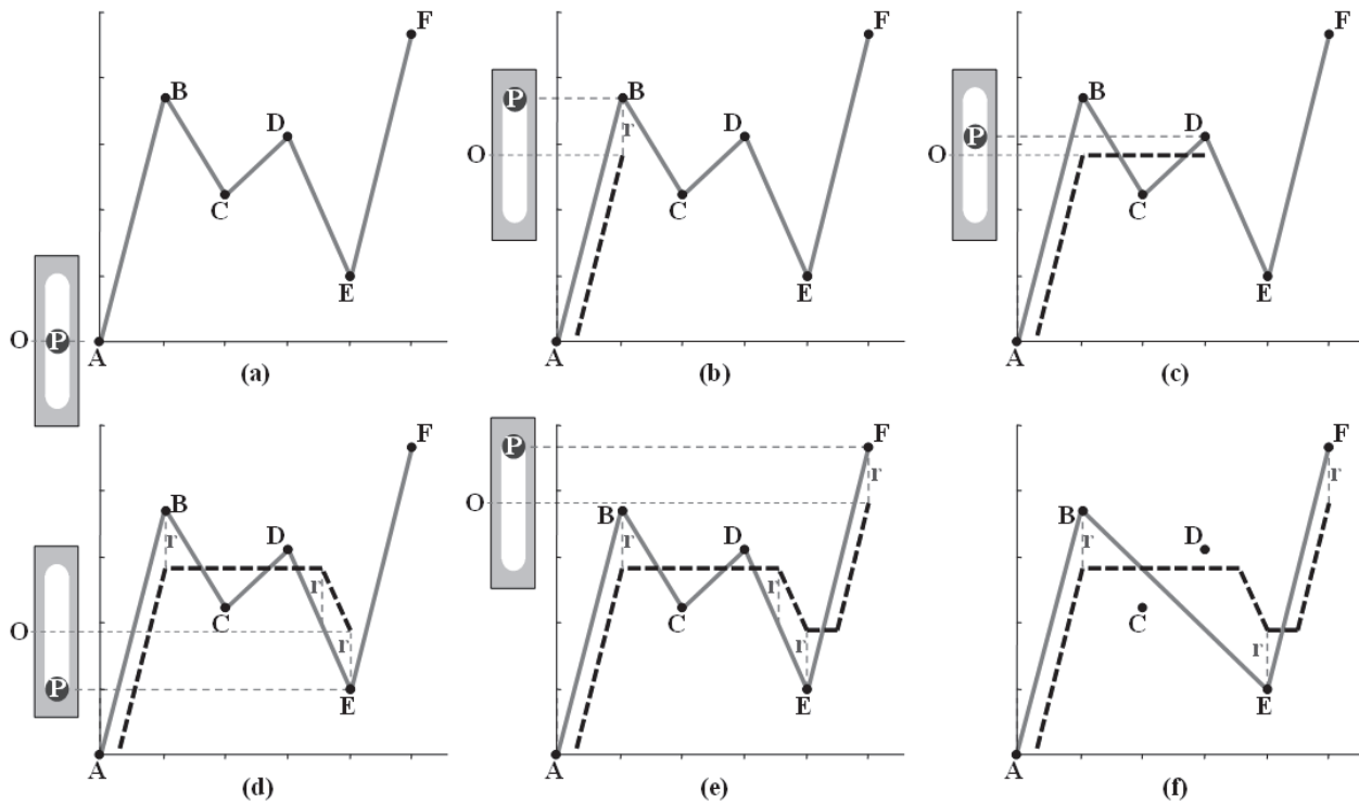
Figure 1: Analogy between the uniaxial racetrack filter and a peg P oscillating inside a slotted plate with center O and slot range 2r . The peg oscillates following the original history, resulting in translations of O represented by the dashed line.
