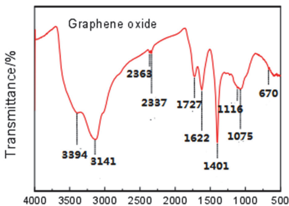
Figure 2: The FTIR spectrum of graphite oxide.
