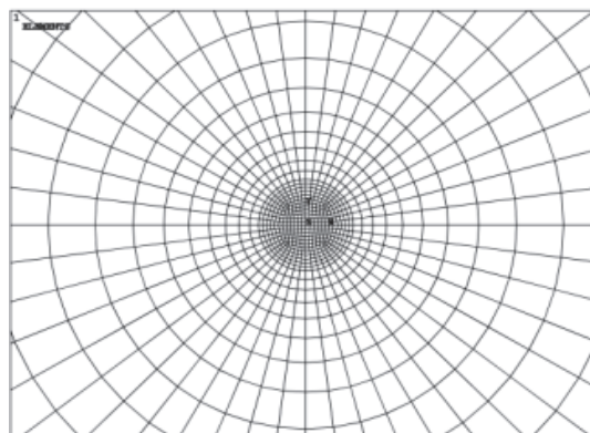
Figure 2: Crack tip finite element mesh.
