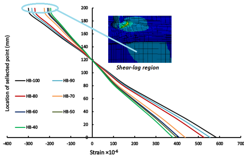
Figure 6: Strain changes at mid-span of the tested beams.
