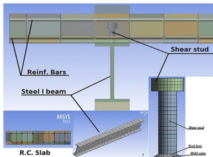
Figure 2: The finite element model used in the study.
