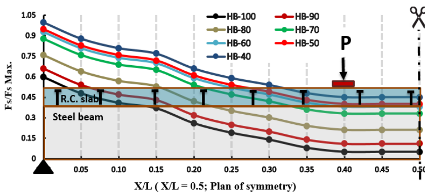
Figure 7: Ratio of stud forces to its relative position.
