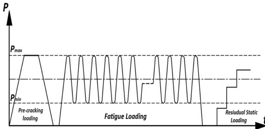
Figure 4: Used cyclic loading pattern [9].
