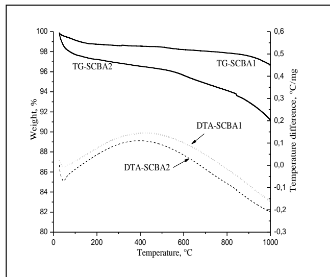
Figure 3. Thermal Analysis for SCBA1 and SCBA2 under inert condition (nitrogen gas)
