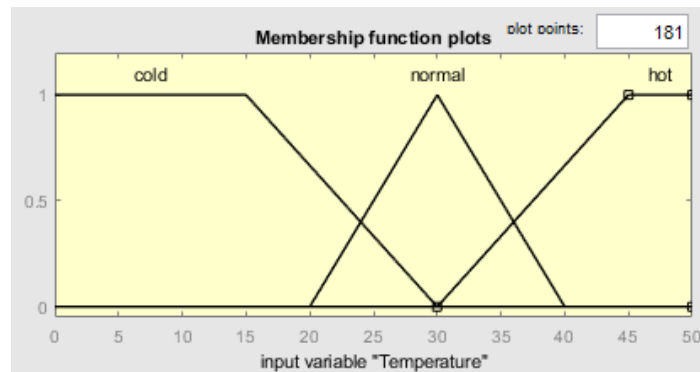
Figure 5. Temperature membership value
