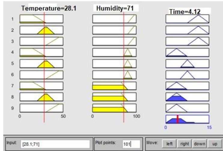
Figure 7. Calculations using Matlab
