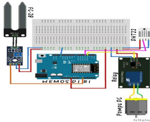
Figure 4. Hardware Circuit Wiring
