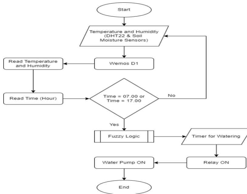
Figure 3 . System Workflow
