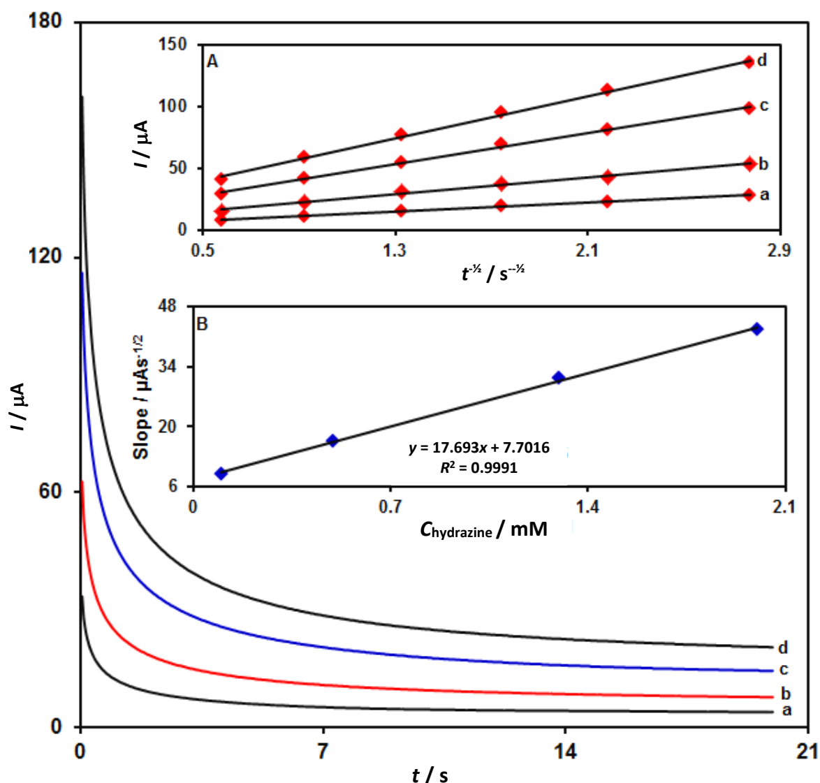
Figure 5. The chronoamperograms obtained at \text{MnO}_2 NRs/SPGE in 0.1 M PBS at pH of 7.0 for different concentrations of hydrazine. Noted that a–d related to 0.1, 0.5, 1.3, and 2.0 mM of hydrazine Inset A: the I plot versus t^{-1/2} observed by chronoamperograms a to d. Inset B: slope plot of the straight line vs. concentration of hydrazine
