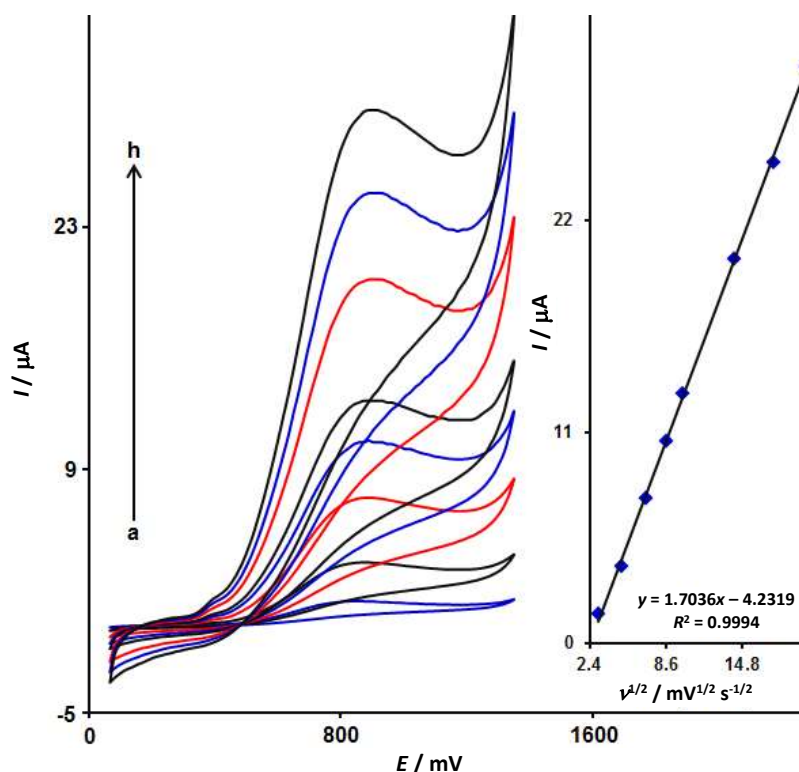
Figure 3. CV curves of 100.0 μM hydrazine in 0.1 M PBS (pH 7.0) at a scan rate of 10 to 400 mV s -1 at MnO 2 NRs/SPGE (a-h refers to 10, 25, 50, 75, 100, 200.0, 300.0 and 400.0 mV s -1 ) Inset: Plot of the square root of the scan rate vs. the oxidation peak current of hydrazine
