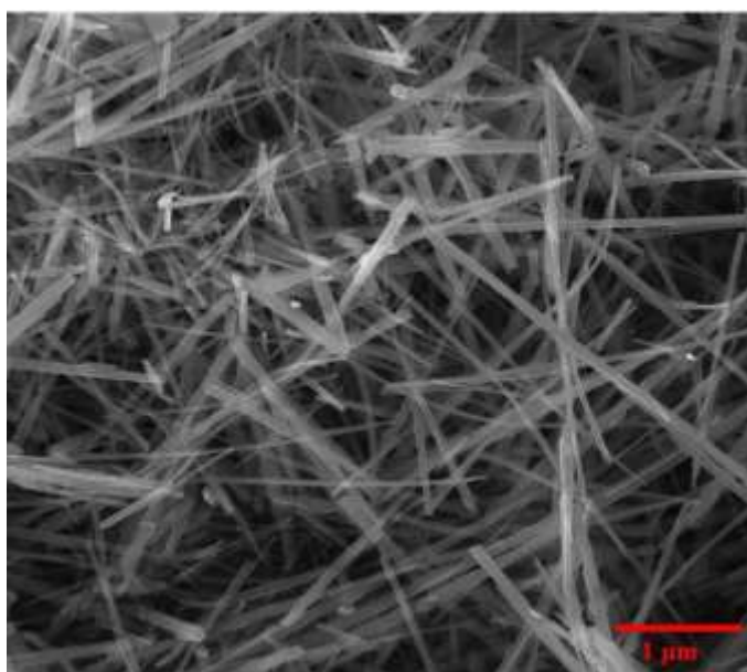
Figure 1. The FESEM images of synthesized MnO 2 nanorods
