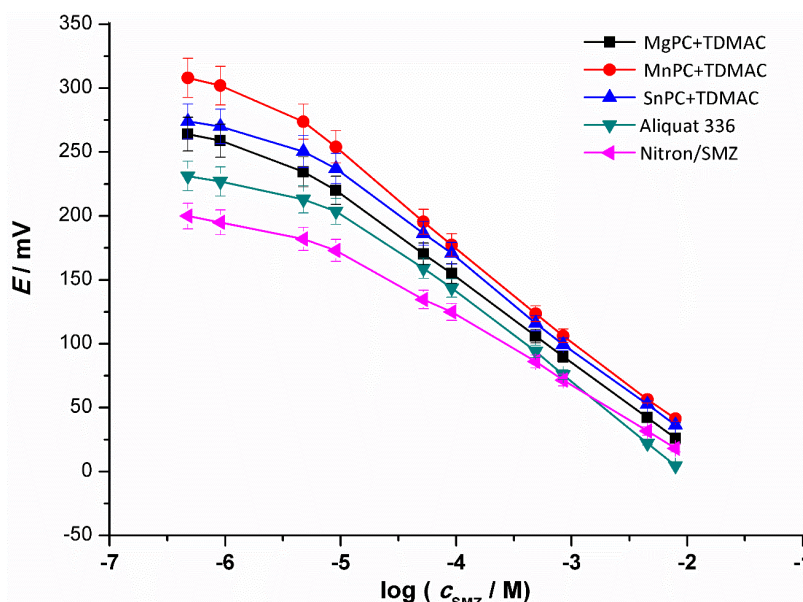
Figure 2. Potentiometric response of SMZ membrane based sensors using 0.01 M Na 2 SO 4 at pH 7
