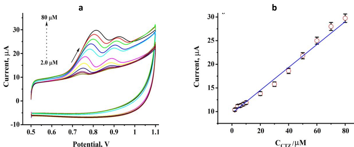
Figure 8. (a) CV responses (0.1 V/s) for CTZ concentrations from 2.0-80 μM at PVLMCNTPS in 0.1 M PBS, pH 7.0; (b) calibration plot of CTZ.
