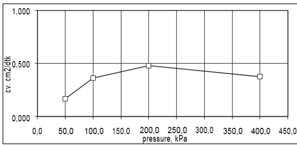
Fig 7. Data Graph of Consolidated Coefficient Analysis Results
