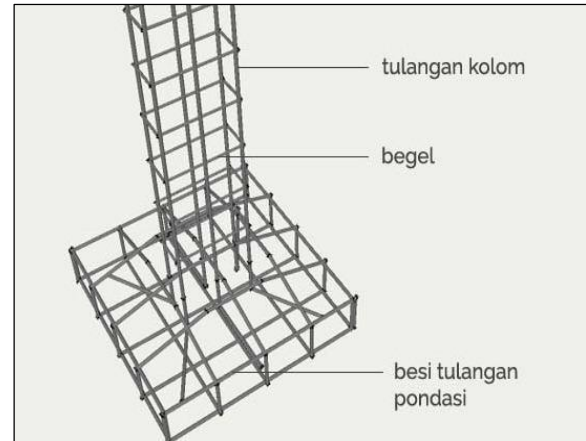
Figure 12. Example of chicken claw foundation modeling
