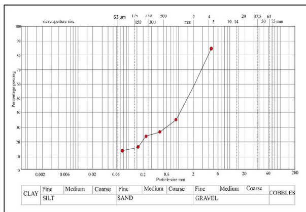
Fig 4. Graph of bore hole 06 sieve analysis
