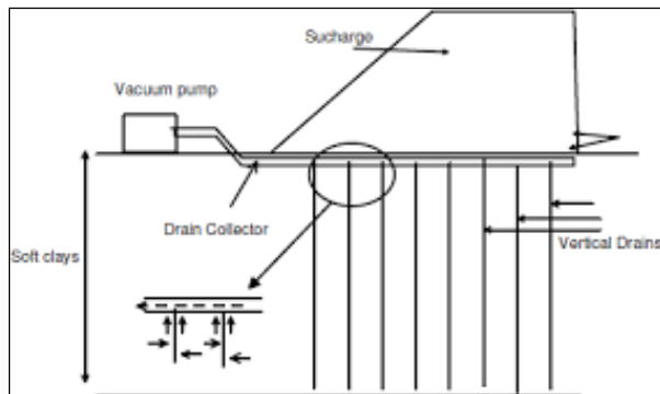
Fig 11. Example of Vertical Wick Drain Modeling
