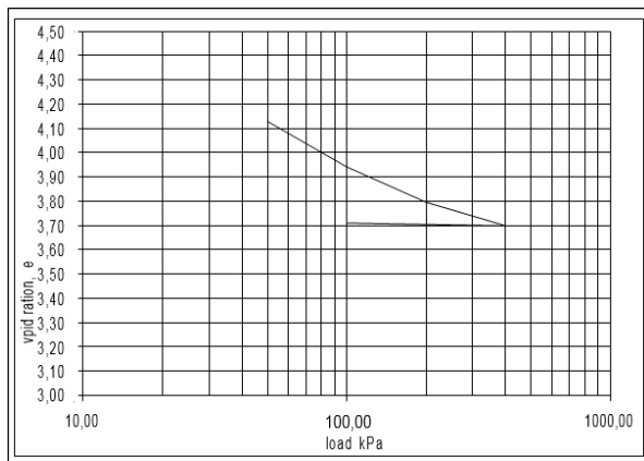
Fig 8. Graph of Compression Coefficient Analysis Results
