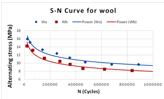
Figure 17. S-N curve of the wool composites
