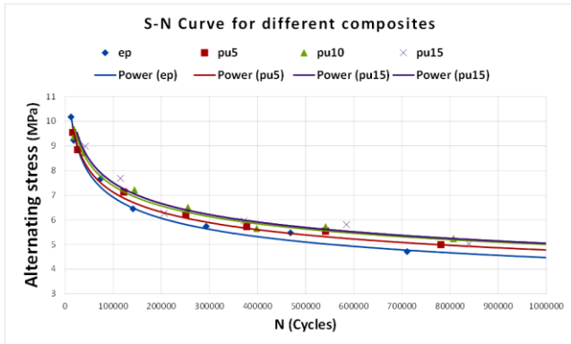
Figure 16. S-N curve of different composites
