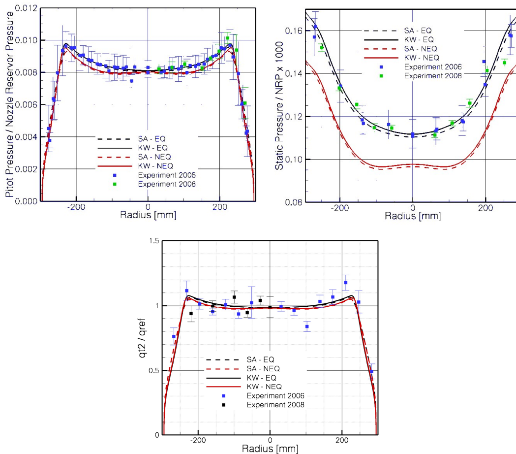
Figure 10: Comparison of measured and computed normalized Pitot pressure (left), static pressure (middle) and stagnation point heat flux distributions at the nozzle exit plane; NEQ: thermal non-equilibrium, EQ: thermal equilibrium, SA: Spalart-Allmaras turbulence model, KW: Wilcox k-\omega turbulence model, NRP: Nozzle reservoir pressure (HEG operating condition H3.3R3.7).
