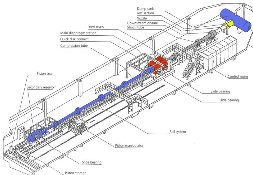
Figure 2: Schematic of the High Enthalpy Shock Tunnel Göttingen, HEG.
