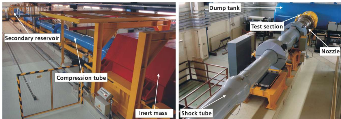
Figure 3: Photographic views of the High Enthalpy Shock Tunnel Göttingen, HEG.
