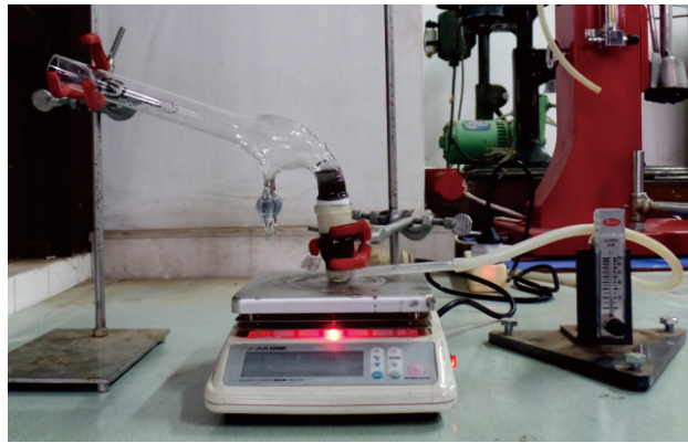
Fig 2 Photograph of a modified Hallimond Tube used for microflotation test.
