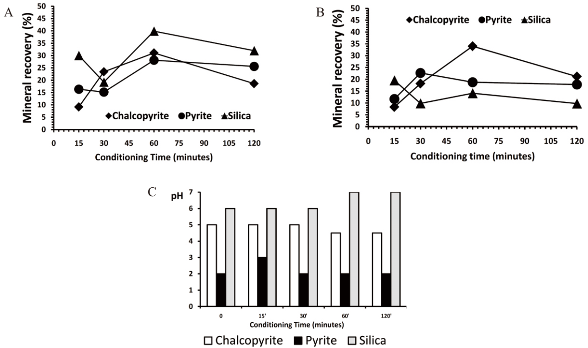
Fig 4 Flotation recovery (%) of chalcopyrite, pyrite, and silica at varying conditioning times with cell concentration of the bacterium Bacillus pumilus strain SKC-2 ( 2.8 \times 10^9 CFU g^{-1} mineral) (A). Flotation recovery (%) of chalcopyrite, pyrite, and silica at varying conditioning times with cell concentration of the bacterium Citrobacter youngae strain SKC-4 ( 2.8 \times 10^9 CFU g^{-1} mineral) (B). The pH values of the bacterial suspension of the bacterium C. youngae strain SKC-4 after chalcopyrite, pyrite, and silica were conditioned with bacterial cells of C. youngae in the microflotation of chalcopyrite, pyrite, and silica (C).
