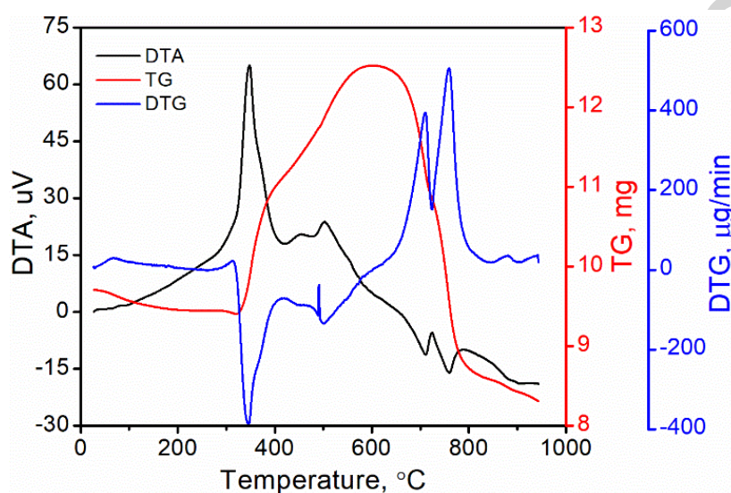
Fig. 2. Thermogravimetric analysis of copper-containing leaching residue
