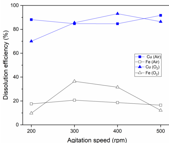
222 Fig. 6. Copper and iron dissolution efficiency as a function of agitation speed (air: 60 min, S/L ratio 200 1:50, 25 °C; oxygen: 30 min, S/L ratio 1:50, 25 °C)
