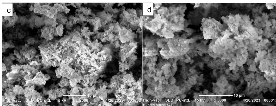
Fig. 13. SEM micrographs of leaching residue; a) water leaching residue of air roasted sample b) acid leaching residue of air roasted sample; c) water leaching residue of oxygen roasted samples, d) acid leaching residue of oxygen roasted samples
