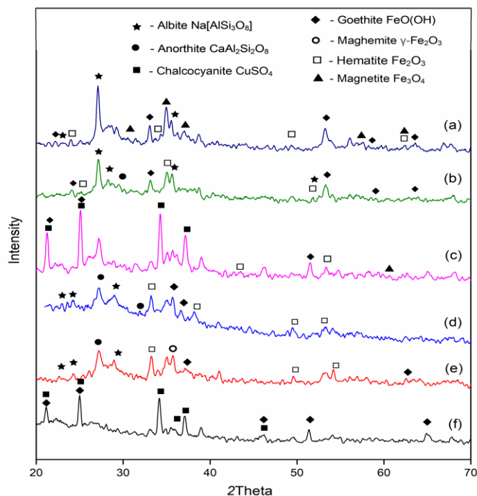
300 Fig. 12. XRD analysis of leaching residue compared with the roasted sample. a) acid leaching residue (O 2 roasted), b) water leaching residue (O 2 roasted), c) oxygen roasted sample, d) acid leaching residue (air roasted), e) water leaching residue (air roasted), and f) air roasted sample
