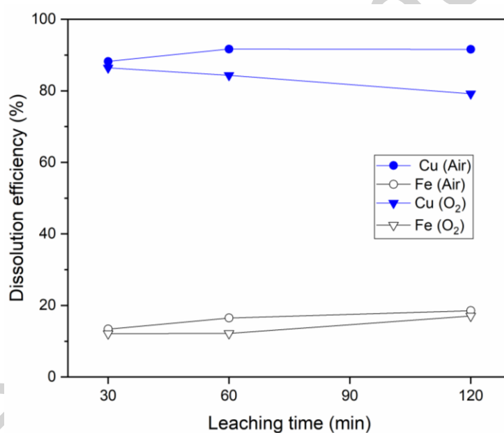
219 Fig. 5. Copper and iron dissolution efficiency as a function of leaching time (S/L ratio 1:50, 500 rpm, 25 °C)
