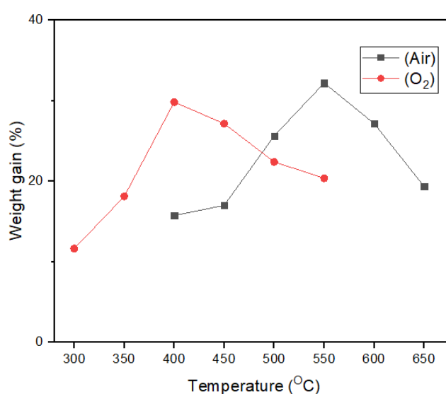
192 Fig. 3. Weight gain vs. the roasting temperature under the air and oxygen roasting (roasting time is 60 mins)
