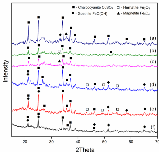
195 Fig. 4. XRD analysis for effect of roasting time at optimum temperature (at 400 °C, O 2 roasted for 180 min (a) 120 min (b) 60 min (c); and at 550 °C air roasted for 180 min (d) 120 min (e) 60 min (f))
