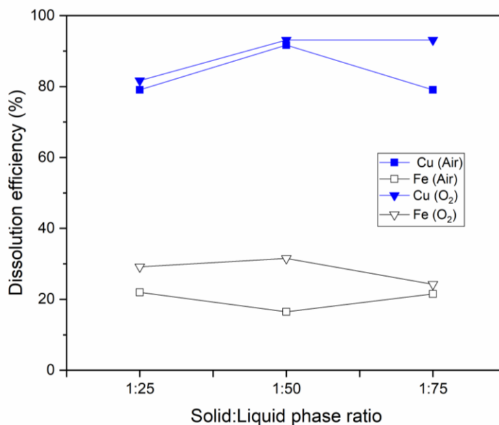
240 Fig. 7. Copper and iron dissolution efficiency as a function of solid-to-liquid phase ratio (air: 60 min, 500 243 rpm, 25 °C; oxygen: 30 min, 400 rpm, 25 °C)
