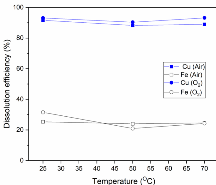
249 Fig. 8. Copper and iron dissolution efficiency as a function of temperature (air: 60 min, S/L ratio 1:50, 500 rpm; oxygen: 30 min, S/L ratio 1:50, 400 rpm)
