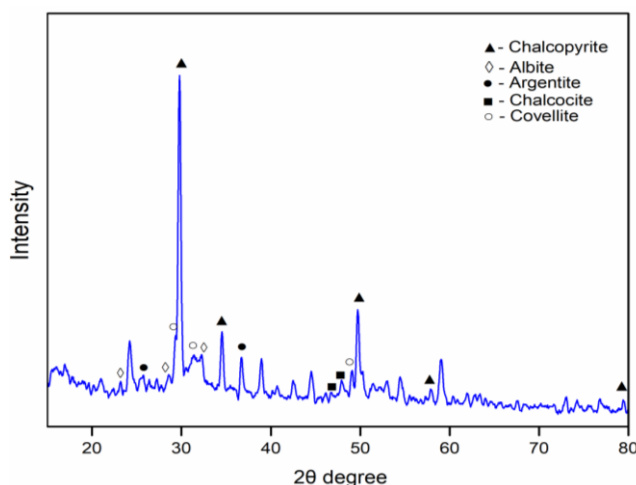
Fig. 1. XRD analysis of copper-containing leaching residue
