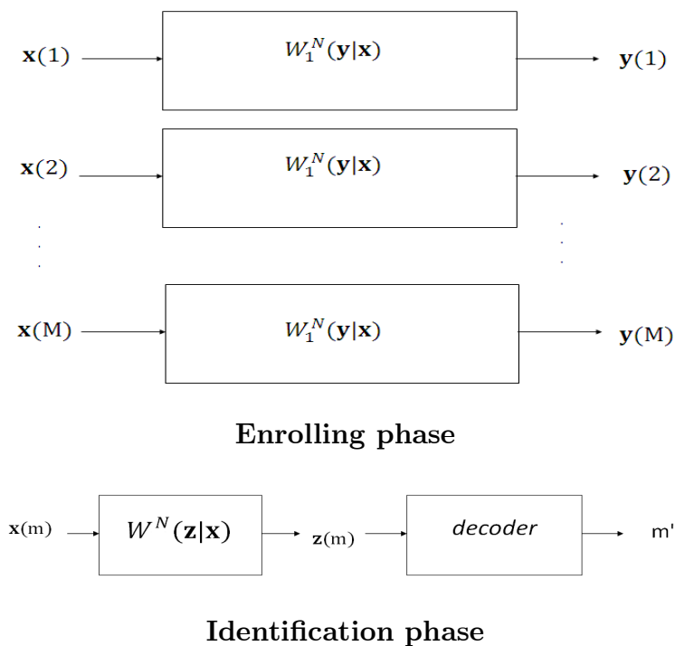
Figure. 1. Model of biometric identification system
