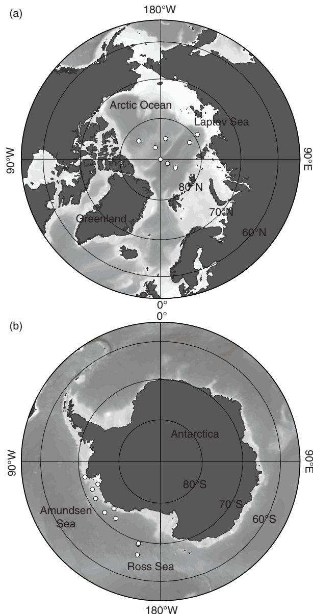
Fig. 1 Locations of sampling sites (white dots) in the (a) Arctic Ocean and the (b) Southern Ocean.
